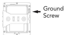
Figure 10: Connect good earth ground to AP here
