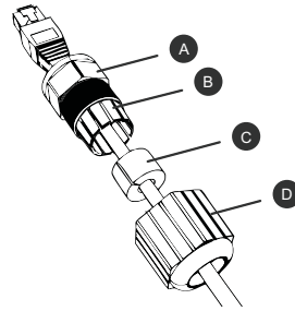
Figure 4: RJ-45 cable and cable gland assembly
