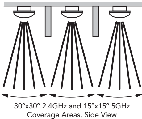
Figure 3: Typical AP high-density narrow-sector coverage
