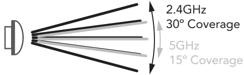
Figure 2: Typical AP narrow sector or point-to-point coverage
