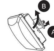
Figure 5: Removing the mounting bracket
